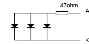
LED Backlight Circuit
