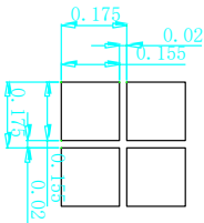
Detail A (20:1)
